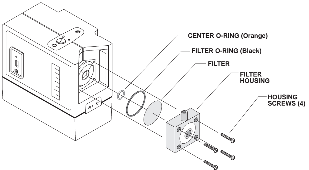
Figure 3.2 Internal Filter Maintenance
