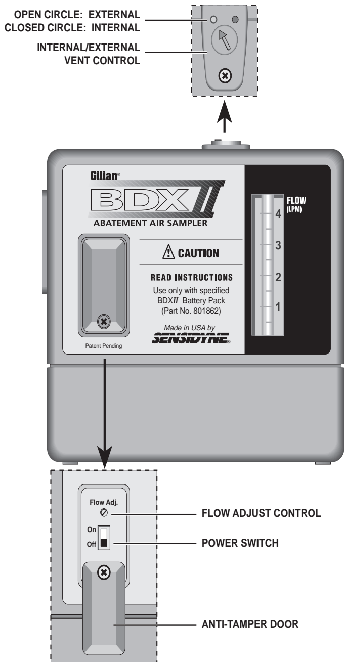
Figure 1.1 BDXII Abatement Air Sampler (Front view)
